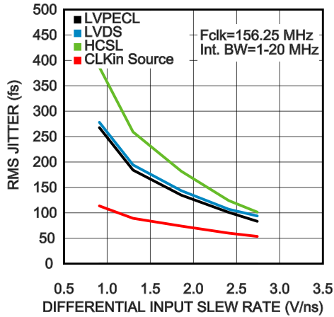
RMS Jitter vs. CLKin Slew Rate @ 156.25 MHz (Note 25)
