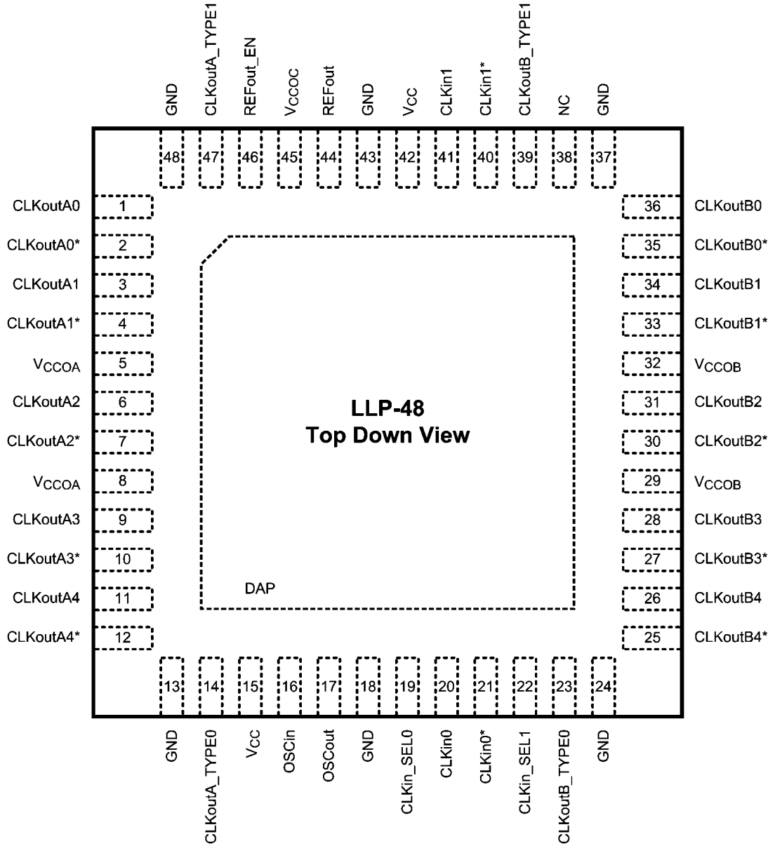
48-Pin LLP Package
