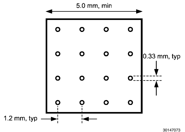
FIGURE 17. Recommended Land and Via Pattern
