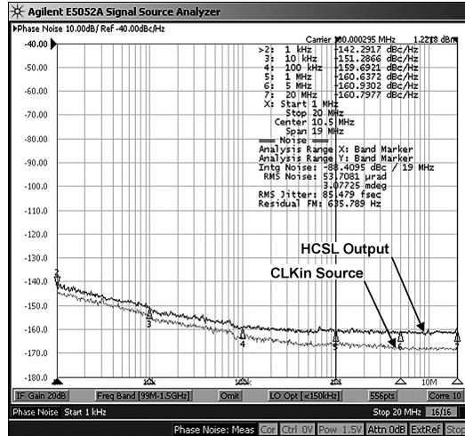
HCSSL Phase Noise @ 100 MHz (Note 25)
