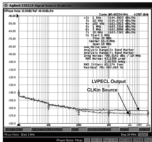
LVPECL Phase Noise @ 100 MHz (Note 25)
