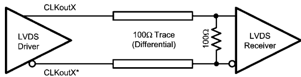
FIGURE 7. Differential LVDS Operation, DC Coupling, No Biasing by the Receiver
