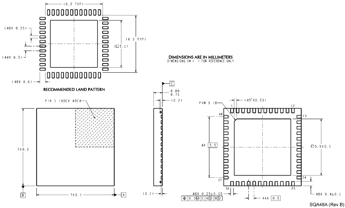
48 Pin LLP (SQA48A) Package
