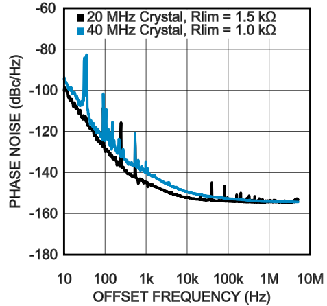
LVDS Phase Noise in Crystal Mode (Note 26, Note 27)
