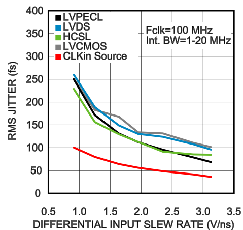
RMS Jitter vs. CLKin Slew Rate @ 100 MHz (Note 25)
