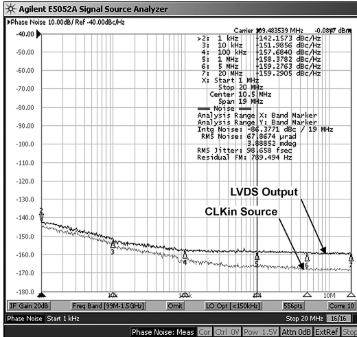
LVDS Phase Noise @ 100 MHz (Note 25)
